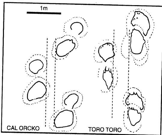
Figure 4. Comparison of sauropod trackways from Cal Orcko (Maastrichtian) and Toro Toro (Campanian).
