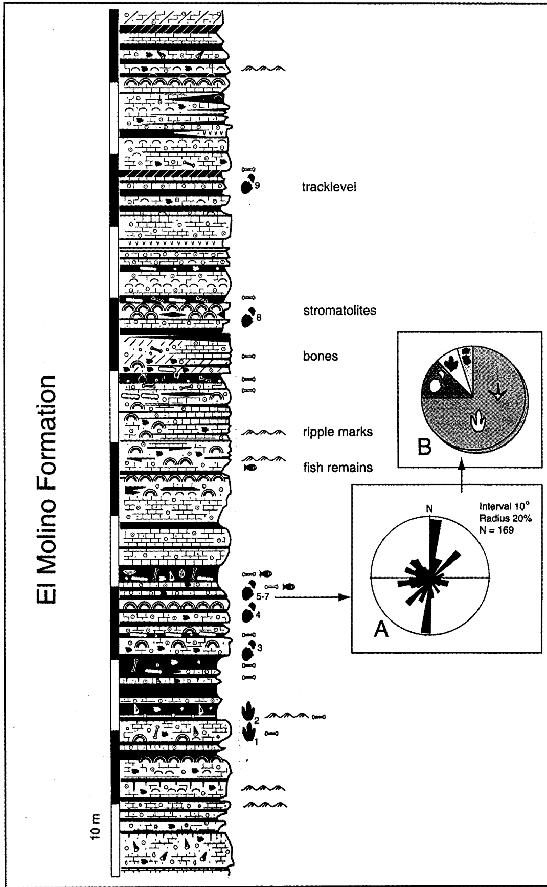
Figure 3. Part of the section at the Cal Orcko quarry showing dinosaur track levels and occurrence of other vertebrate remains. A, rose diagram of dinosaur trackways of level 5. B, ichnotaxonomic composition of tracklevel 5.
