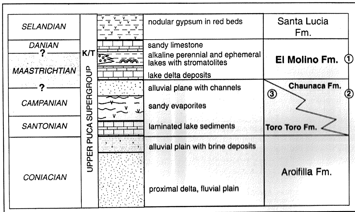
Figure 2. Litho- and chronostratigraphic context of study area: 1, Cal Orcko; 2, Humaca; 3, Toro Toro.
