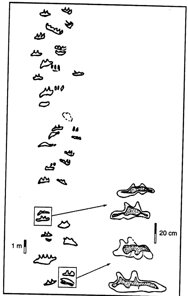
Figure 5. Trackway of an ankylosaur (n° T 4/5/1) from Cal Orcko (level 4) with inset of detailed morphology.
